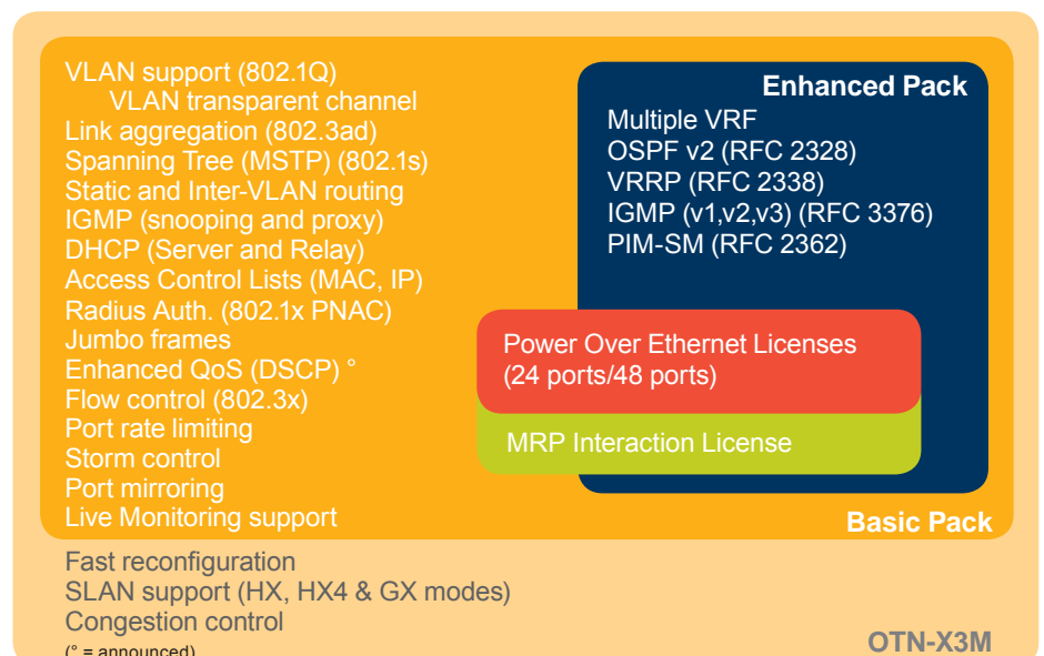
Figure 2: Feature Packs
